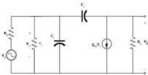
Fig. 2. High-frequency equivalent half-circuit
