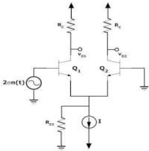
Fig. 1. Differential amplifier with one end grounded
