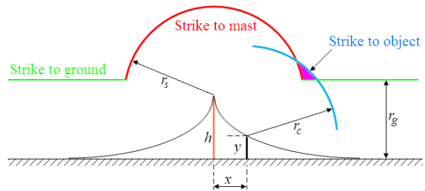
Fig. 1. Striking distances
