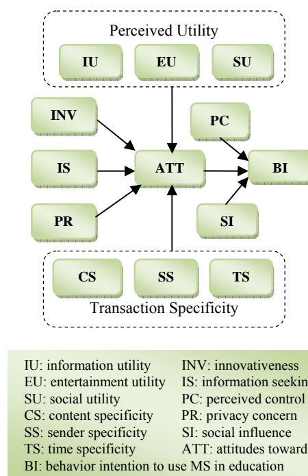
Fig. 1 Determinants of students' intentions to use the university's mobile messaging service.
