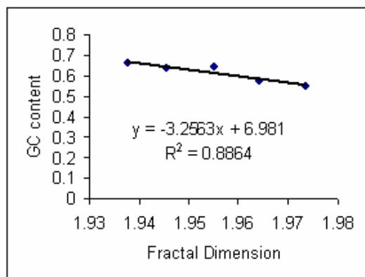
Fig. 7 Fractal dimension versus sequence GC content for the studied five archaea-eyryarchaeota thermophiles
