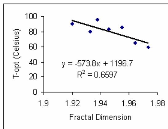
Fig. 4 Fractal dimension versus T-opt (optimal growth temperature) for the studied five archaea-eyryarchaeota thermophiles and two arachea-crenarchaeota thermophiles.
