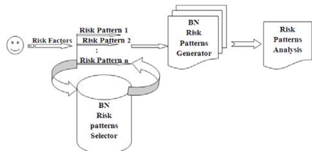
Fig. 5.The WPRiMA architecture
