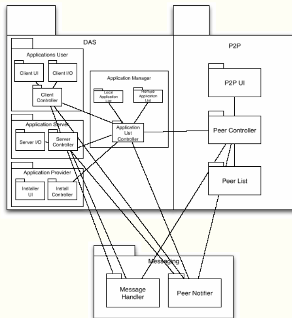
Fig. 1. CPCC architecture
