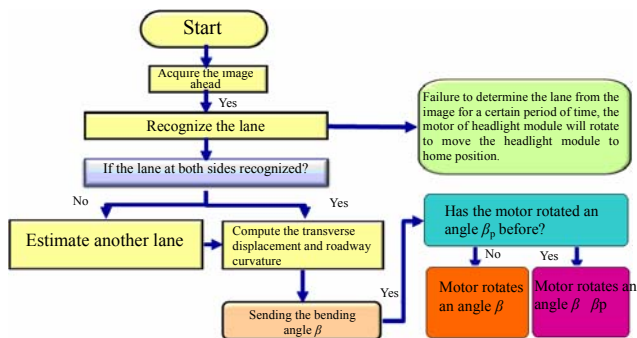
Fig. 7 Flowchart for bending control of headlight
