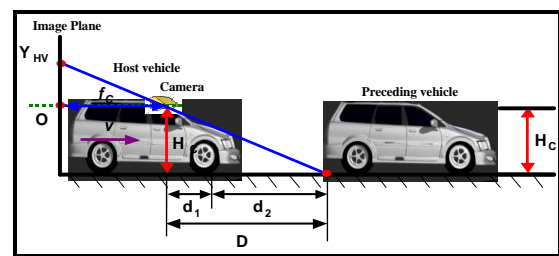
Fig. 6 Headway distance estimation model
