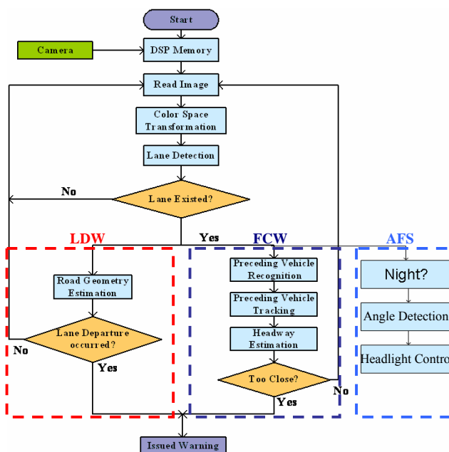
Fig. 2 Flowchart of the integrated vehicle image system
