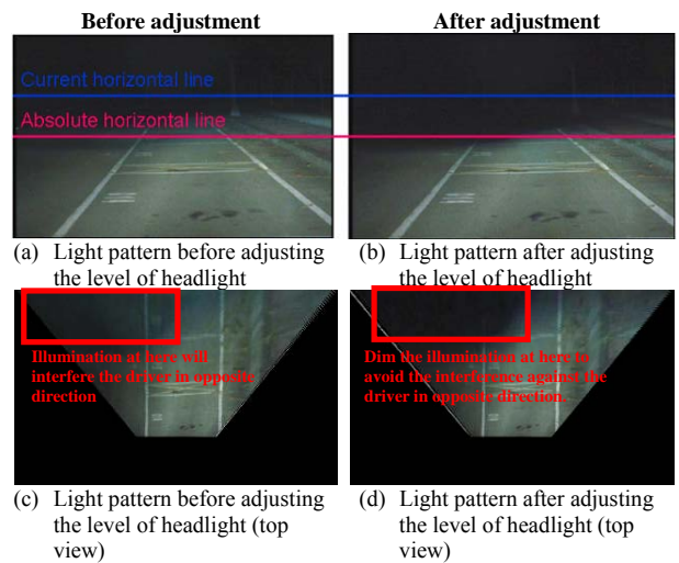
Fig. 11 Variations of light pattern for level adjustment of headlight
