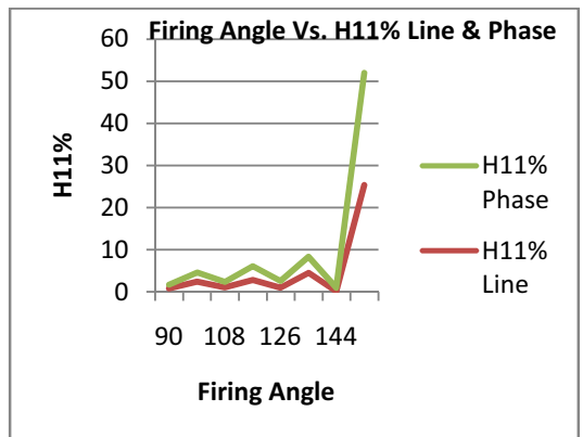
Fig.14(c) Odd harmonics of TCR for H11
