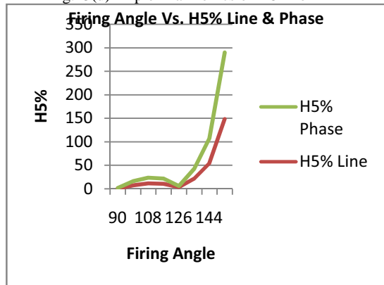
Fig.14(a) Odd harmonics of TCR for H5
