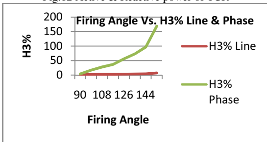
Fig.13(a) Triplen harmonics of TCR for H3
