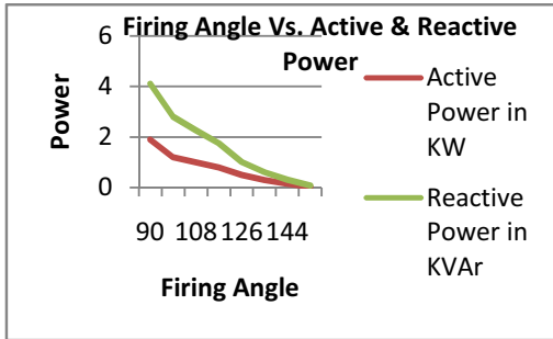
Fig.12 Active & Reactive power of TCR
