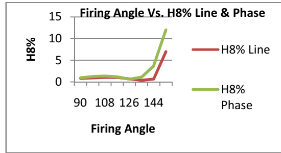
Fig.15(c) Even harmonics of TCR for H8
