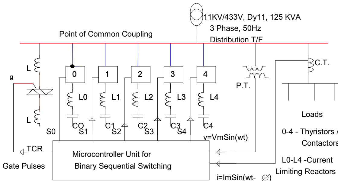
Fig. 1 Basic FC-TCR Scheme
