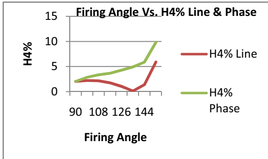
Fig.15(b) Even harmonics of TCR for H4
