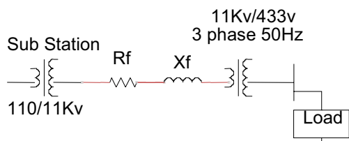
Fig.4 Single Line Diagram of Distribution System
