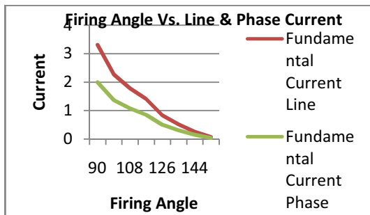
Fig.9 Fundamental component of line & phase current for TCR
