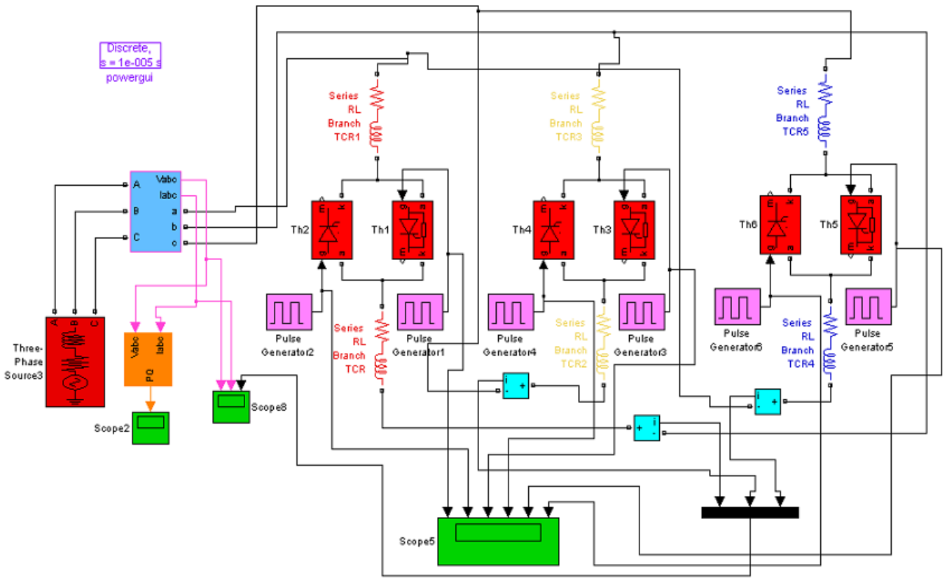
TCR SIMULATION MODEL
