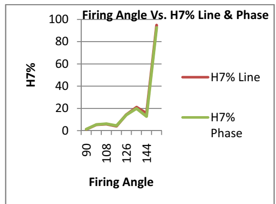
Fig.14(b) Odd harmonics of TCR for H7
