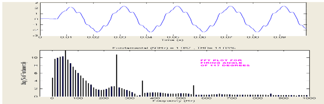
Fig. 6.37 Harmonic spectrum of line current for \alpha = 117^\circ
