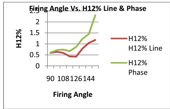
Fig.13(d) Triplen harmonics of TCR for H12
