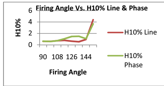
Fig.15(d) Even harmonics of TCR for H10
