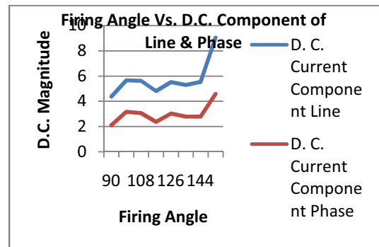
Fig.10 D. C. components of TCR
