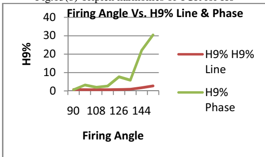
Fig.13(c) Triplen harmonics of TCR for H9
