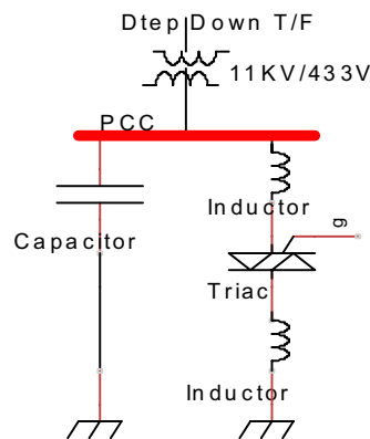
Fig. 6 FC-TCR Scheme
