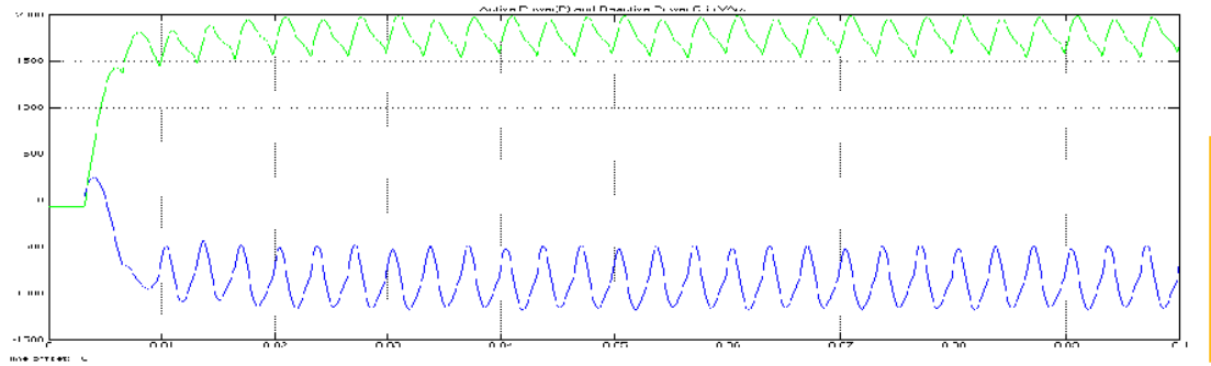
Fig. 17 Active and reactive power for \alpha = 117^\circ
