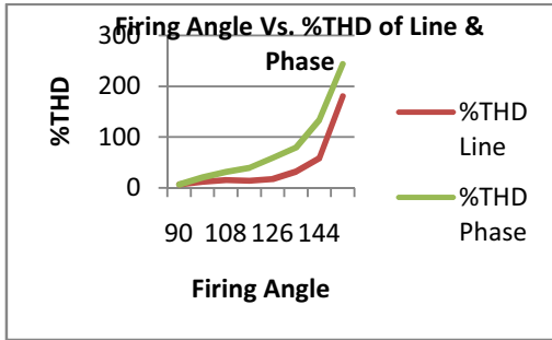
Fig.11 Total THD components of TCR
