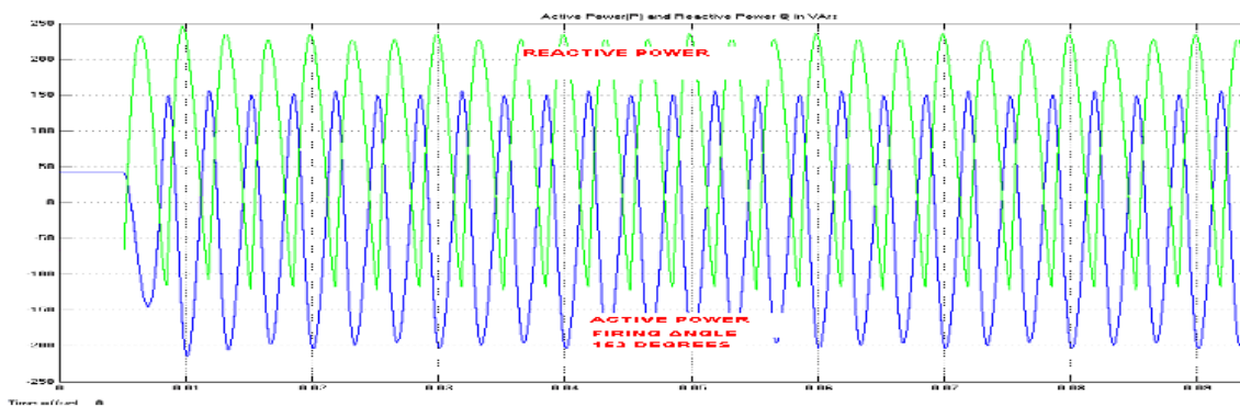
Fig.20 Active reactive power at \alpha = 153^{\circ}
