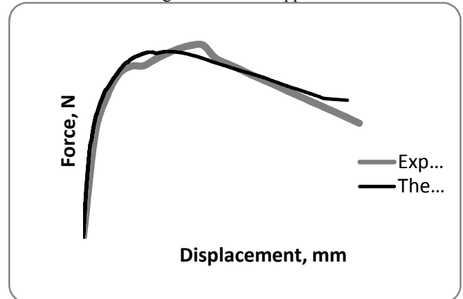
Fig. 7 Load – crack mouth opening displacement (CMOD) diagram for 4 point bending test, SFRHPC with fiber amount 320 \text{ kg/m}^3 (Tabix 50)
