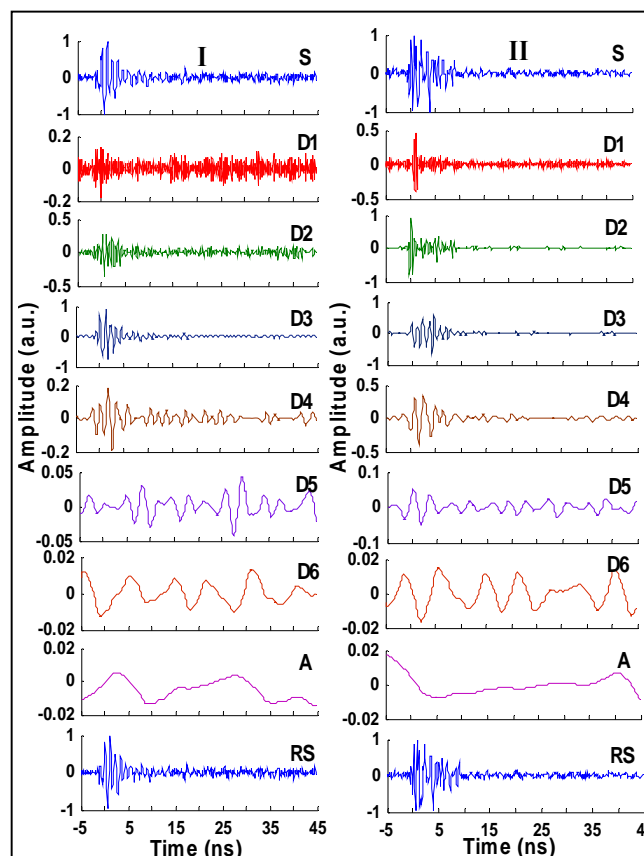
Fig. 13 Typical MRSD analysis of UHF signal (I) UHF signal generated due to particle movement (II) UHF signal generated due to corona D1-D6 are different level of decomposition, (S) actual signal (RS) reconstructed signal
