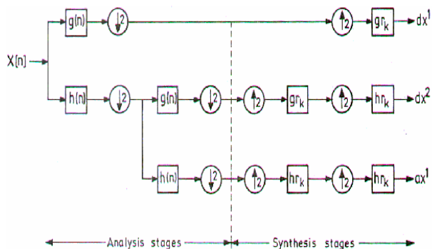
Fig. 4 Schematic representation of implementation of MRSD
