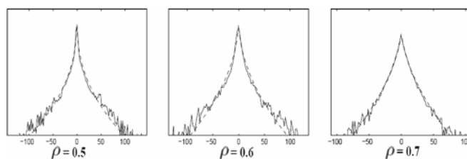
Fig. 4 Coefficient histograms for a single wavelet subband plotted in the log domain. Also shown (dashed lines) are fitted model densities respectively
