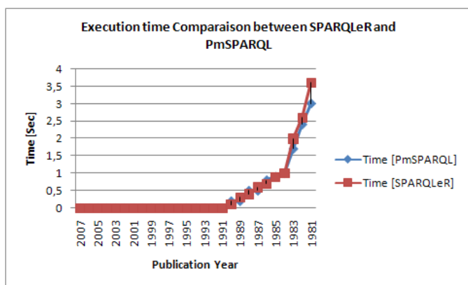
Fig. 8. Execution Time Comparison between SPARQL and PmSPARQL
