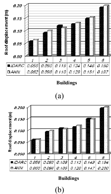
Fig. 5 Roof displacements in two directions; (a) x direction, (b) y direction
