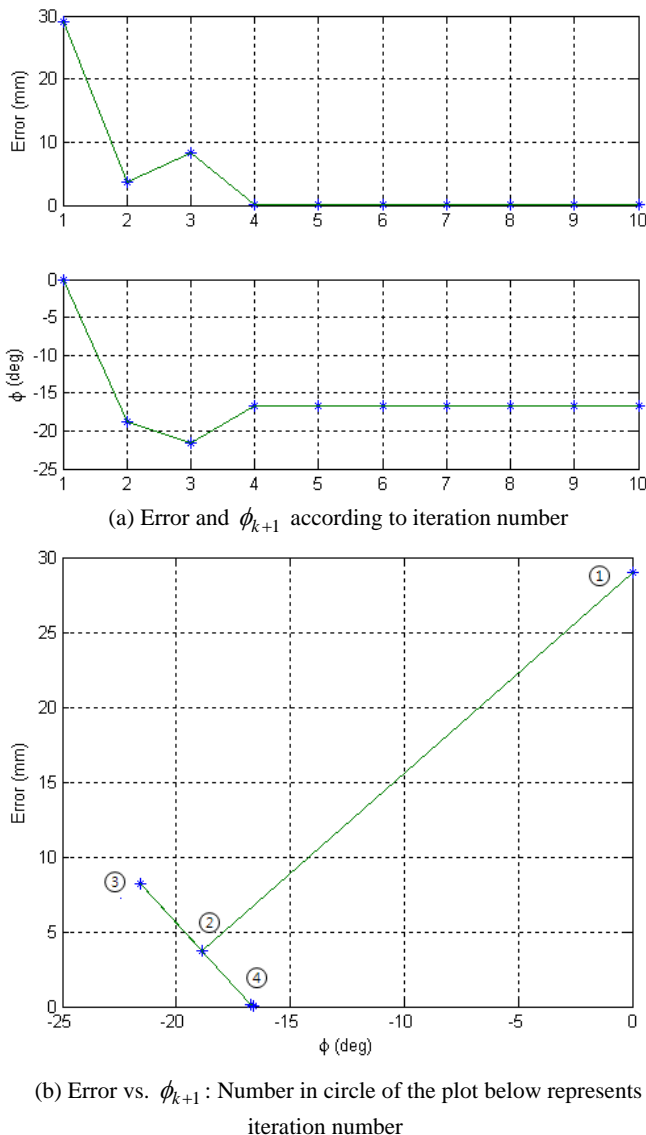
Fig. 8 Simulation results without a reinforced error correction algorithm: Error decreases rapidly as iteration goes
