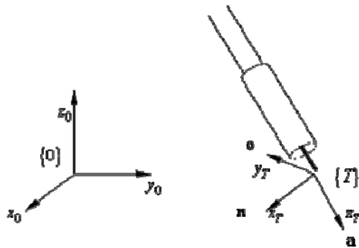
Fig. 5 Vectors related to tool orientation
