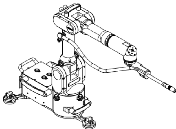
Fig. 1 5-DOF manipulator
