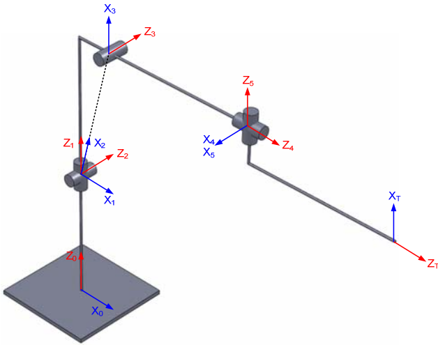
Fig. 2 Definition of frames
