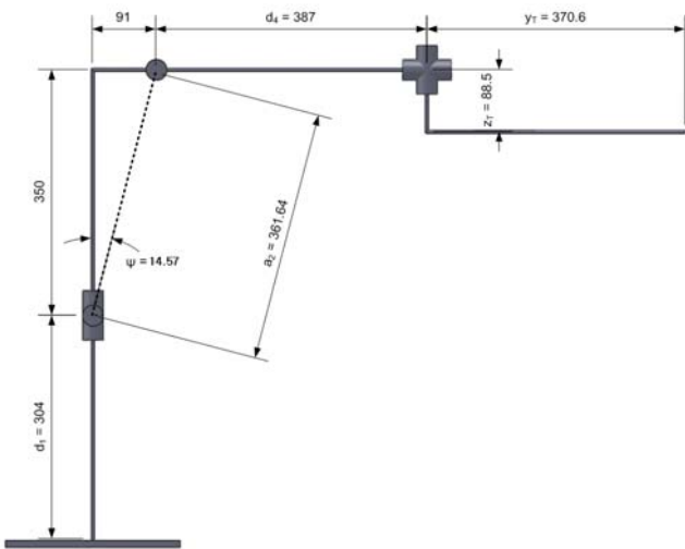
Fig. 3 Length of each link
