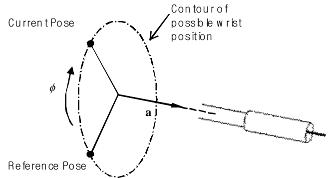
Fig. 6 Possible wrist position and definition of \phi
