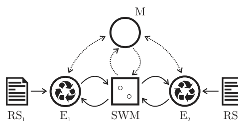
Fig. 1. Web of Inference Systems . WoIS members are inference systems constituted by an inference engine (E) and a rule set (RS) each. SWM is the shared working memory and it is where all the shared facts are stored and accessed by any member of the WoIS. A system, M, plays the role of web manager .
