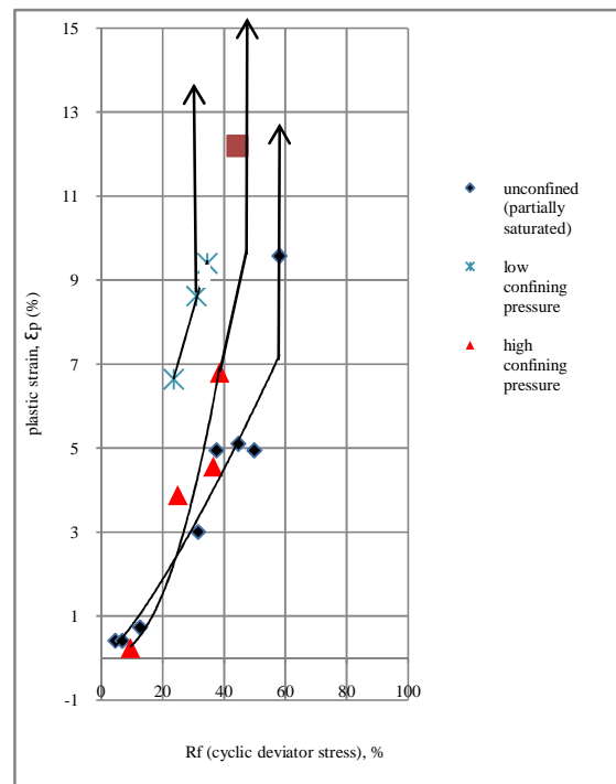
Fig. 5 Plastic strain versus cyclic deviator stress
