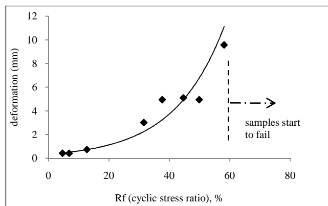
Fig. 1 Deformation of the sample due to cyclic shear loading
