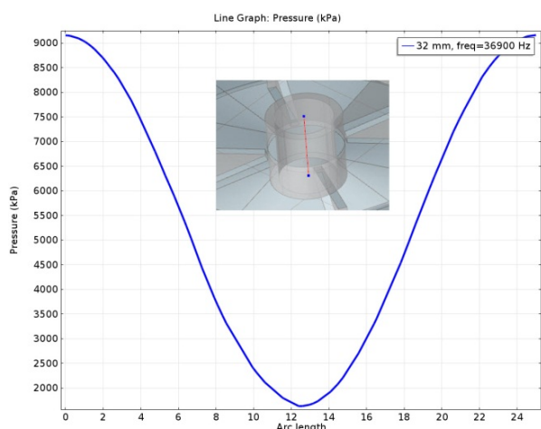
Fig. 9 Acoustic pressure distribution in cylinder with water on resonance frequency (Fig. 3b)
