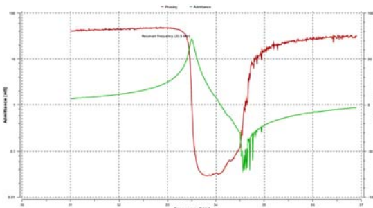
Fig. 10 Admittance-frequency and phase characteristics (free (Fig. 3a))
