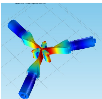
Fig. 5 The distribution of vibration amplitude (Fig. 3a)
