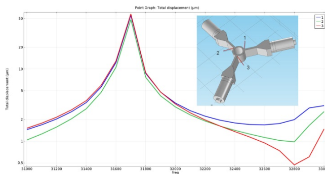
Fig. 4 Total displacement vs. frequency (Fig. 3a)
