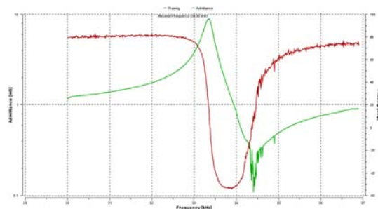
Fig. 11 Admittance-frequency and phase characteristics (loaded (Fig. 3a))
