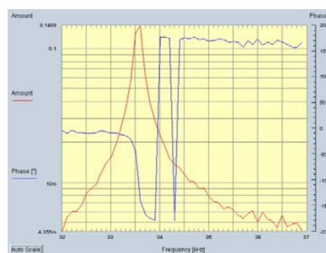
Fig. 12 The complex impedance and phase characteristics of proposed ultrasonic PM system (Fig. 3a)
