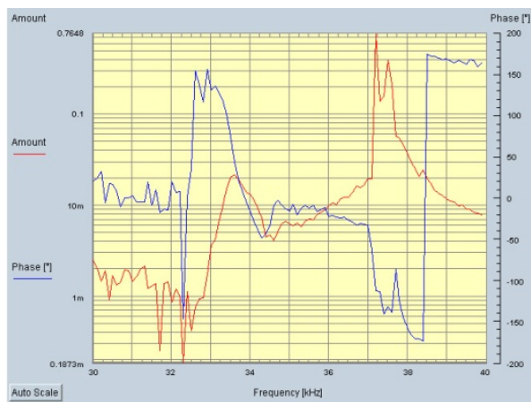
Fig. 15 The complex impedance and phase characteristics of proposed ultrasonic PM system (Fig. 3b)
