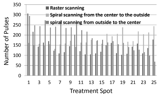
Fig. 5 The pulse number of each treatment spot using different scanning pathway
