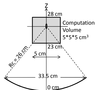
Spherical-focused HIFU transducer Fig. 1 System configuration of the HIFU system
