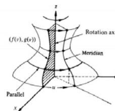
Fig. 1. Surface of revolution [7]
