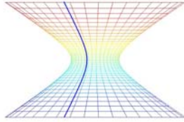
Fig. 3. Meridians on the Hyperboloid are geodesic.
