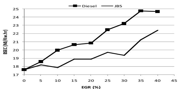
Fig. 5 Variation of BSEC with EGR rates
