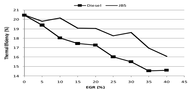
Fig. 3 Variation of thermal efficiency with EGR rates
