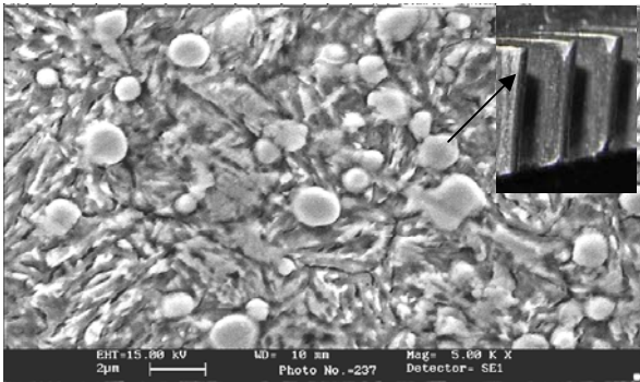
Fig. 5: SEM micrograph of ASP30 hob microstructure
