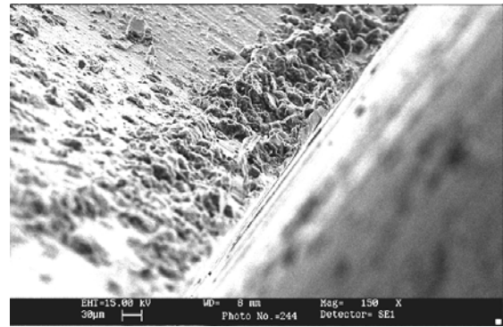
Fig. 2: SEM topography of built-up edge
