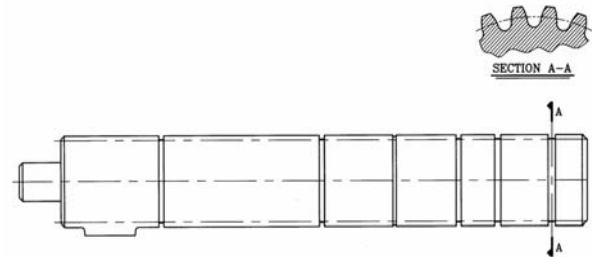
Fig. 1: Main shaft of a tractor as gear blank
