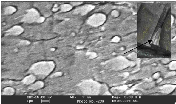
Fig. 6: SEM micrograph of M2 hob microstructure
