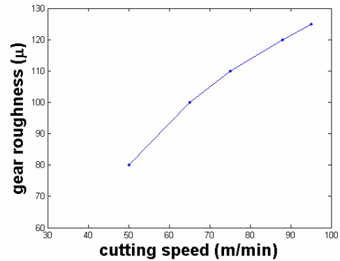
Fig. 8: Surface roughness of gear(μm) vs. cutting speed
