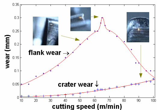
Fig. 3: Flank and crater wear vs. cutting speed
