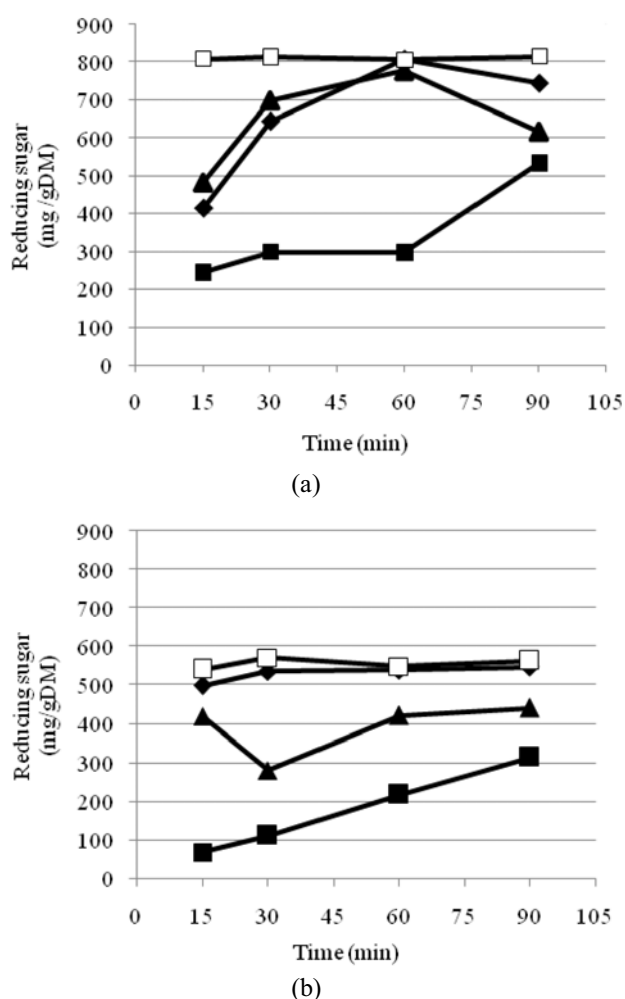
Fig. 3 Effect of temperature on hydrolysis of cassava bagasse to reducing sugar at various times. (a) 0.1 M Sulfuric acid; (b) 0.1 M Phosphoric acid. ( \Delta ) 115°C; ( \blacktriangle ) 120°C; ( \blacksquare ) 125°C; ( \square ) 130°C.
