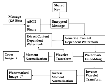
Fig. 2 Proposed watermarking scheme
