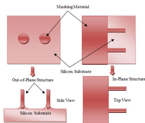
Fig. 1 In-plane and out-of-plane microneedles structure Out-of-plane microneedles are easier to fabricate in arrays.
