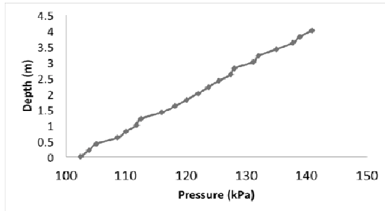
Fig.15 Pressure Data
