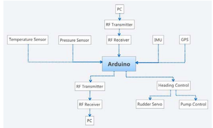
Fig. 7 Automation Control Flow Diagram
