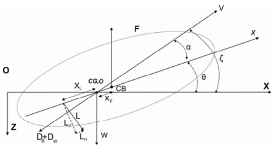
Fig. 12 Simplified FBD During Ascent
