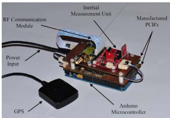
Fig. 6 Main Control Board
