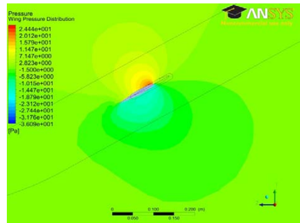
Fig.11 Wing Pressure Distribution
