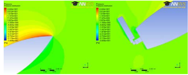
Fig. 9 Pressure Distribution
