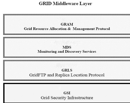
Fig. 5 Grid middleware layer in detail
