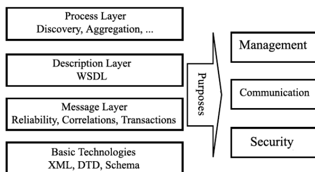
Fig. 3 Web services architecture and its purposes
