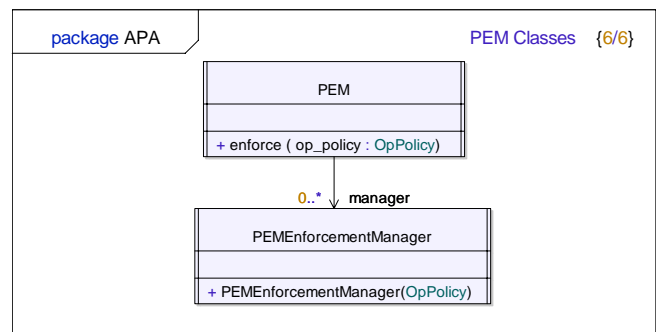
Fig. 8 Class Diagram of the PAM internal components
