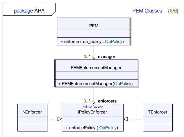
Fig. 9 Class Diagram of the PEM internal components
