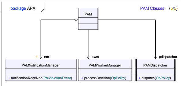
Fig. 6 Class Diagram of the PAM internal components
