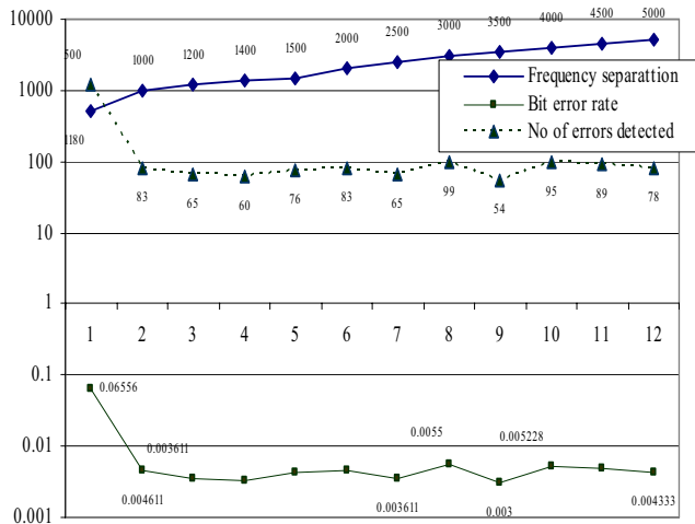
Fig. 6 Bit error rate and Number of errors detected for different frequency separation (Hz).
