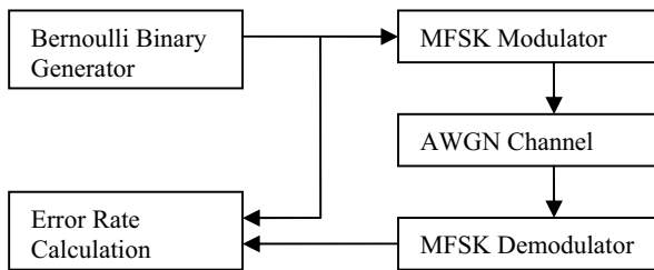
Fig. 2 Communication link model
