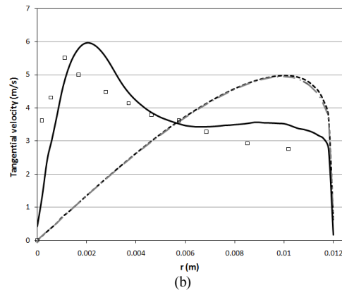
Fig. 3 Tangential velocity profile versus radial position (a: Z=5 cm, b: Z=14cm)
