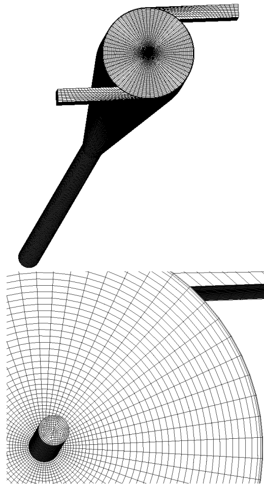
Fig. 2 Generated mesh for hydrocyclone simulations
