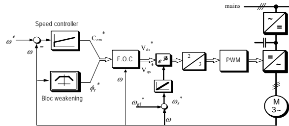
Fig. 2 Block scheme of IFOC on voltage control inverter
