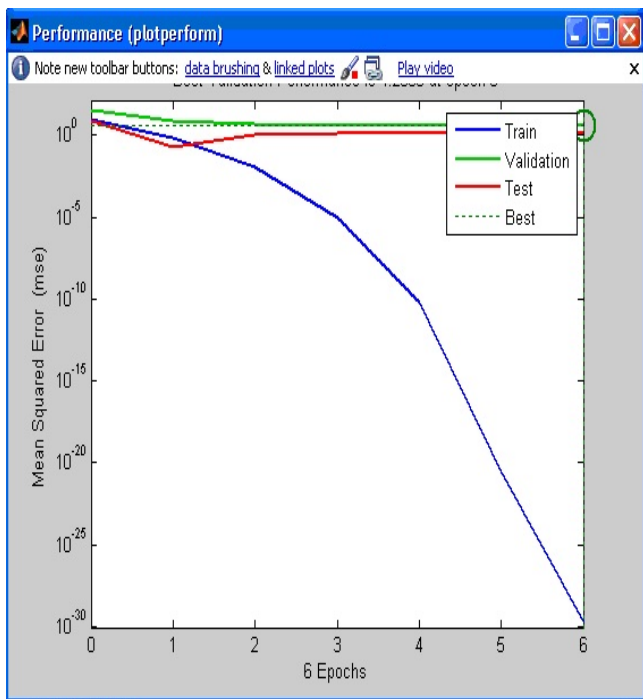
Fig. 2 Mean Square Errors (MSE) in TrainedNWlm
