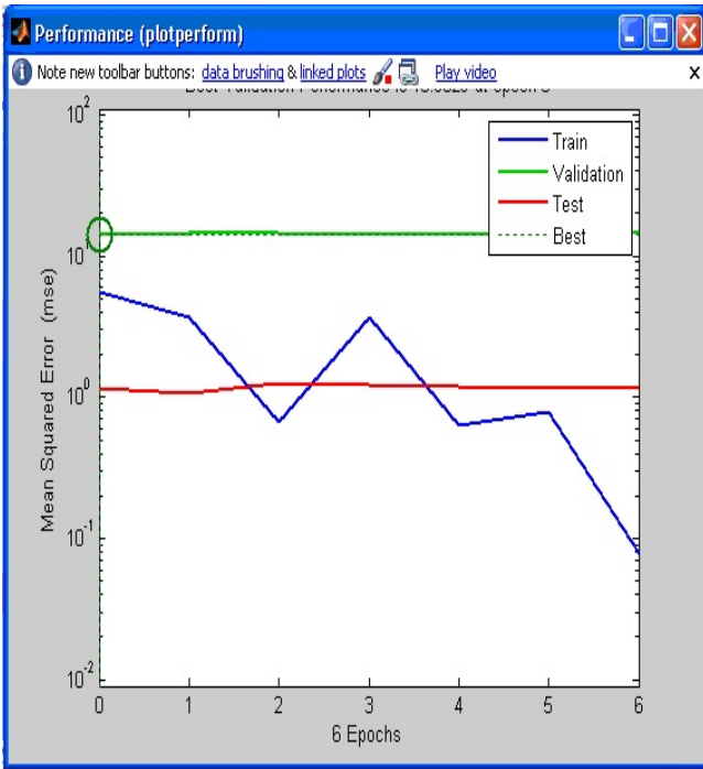
Fig. 6 Mean Square Errors (MSE) in TrainedNWrp
