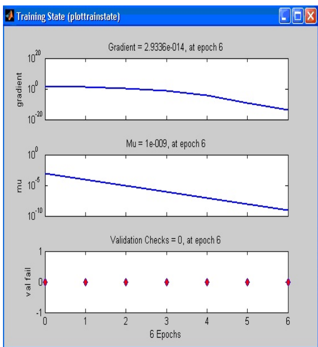
Fig. 3 TrainedNWlm, Training State
