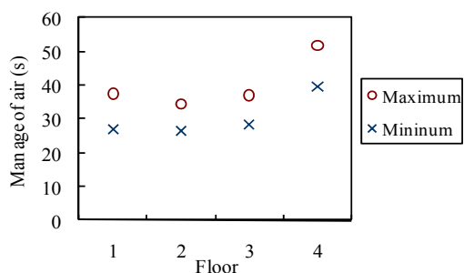
Fig. 5 Maximum and minimum mean age of air due to fenestration combination as a function of floor in the breathing zone
