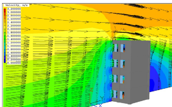
Fig. 4 Outdoor wind field with wind profile function
