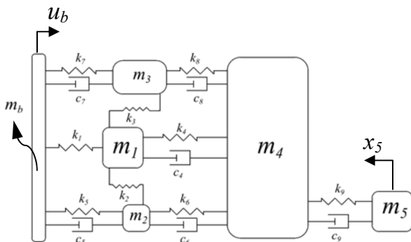
Fig. 12 5-DOF LH model with external excitation
