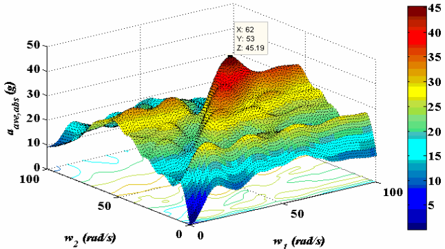
Fig. 15 Absolute average of deceleration of occupant submitted to combination excitation for Dodge Neon
