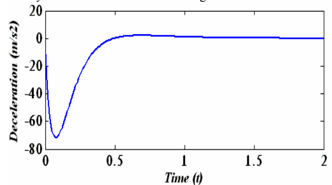
Fig. 2 Deceleration on m_2 in 2 degree of freedom model obtained from analytical solution
