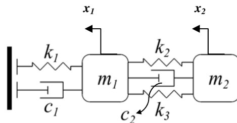
Fig. 1 Two degree of freedom model
