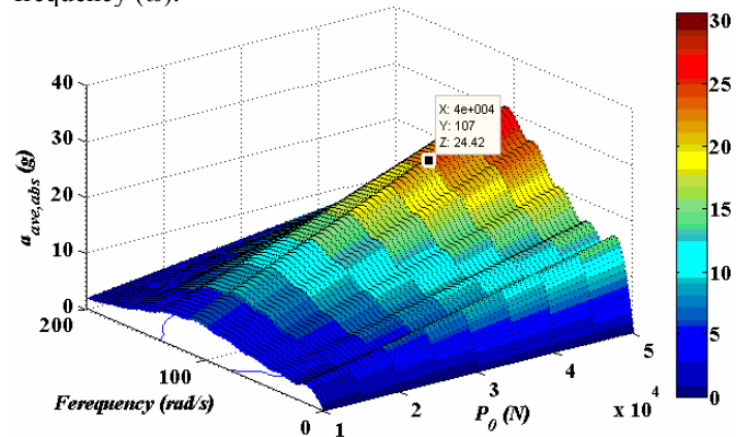
Fig. 13 Absolute average of deceleration of occupant submitted to sin excitation for Dodge Neon
