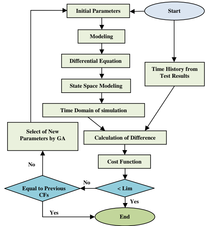
Fig. 5 Algorithm of problem solving
