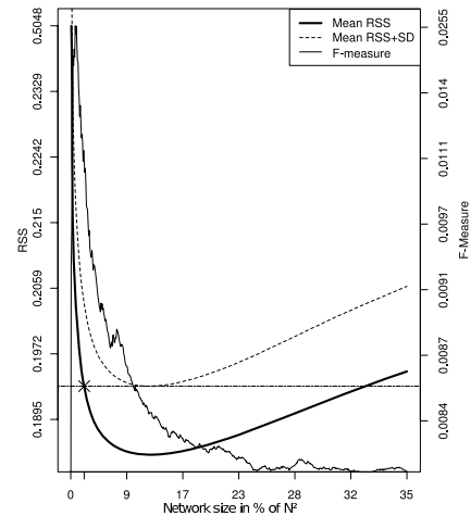
Fig. 1: Optimising the network size for BIND prior-knowledge.
