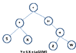
Fig. 5. Example of a parse tree representation.
