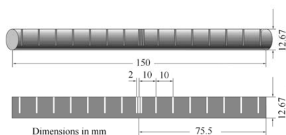
Fig. 2 PMMA cylinder for positioning the TL dosimeters
