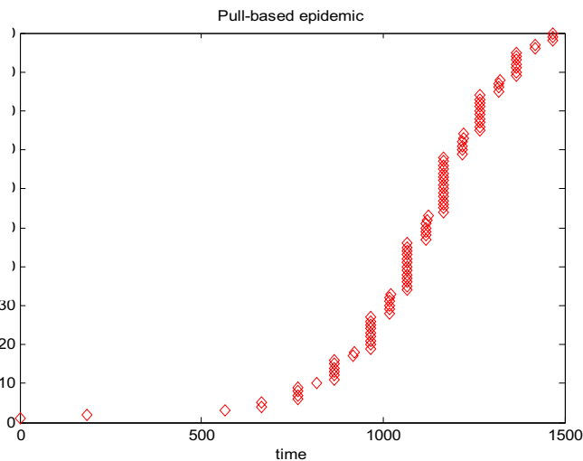
Fig. 3 - Time of infection for each peer, n=100
