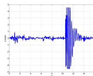
Fig. 2: Sferic: lightning transient with ionospheric echoes
