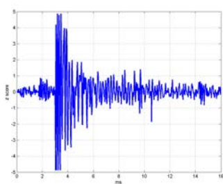
Fig. 4: Tweak: ionospherically dispersed spheric
