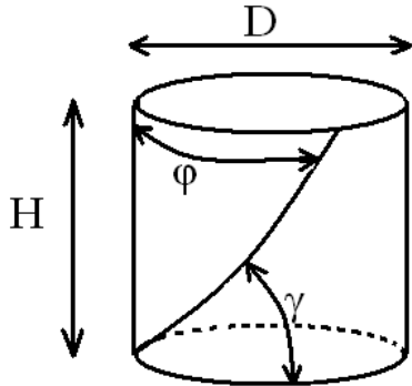
Fig. 1. Geometrical schema of the proposed rotor architecture
