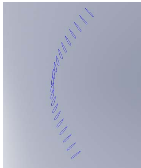
Fig. 4. Airfoil sections determining the 3D architecture of the proposed rotor blade
