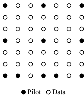
Fig. 2 Pilot distribution for OFDM systems in the frequency-time grid
