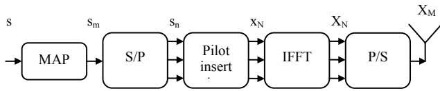
Fig. 1 The transmitter structure of the OFDM system
