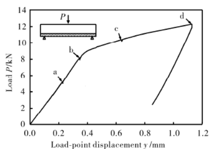
Fig. 5 Load versus load-point displacement curve obtained
