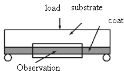
Fig. 4 Schematic of observation location
