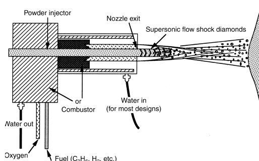
Fig. 1 High velocity oxy fuel Thermal spray process
