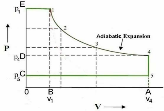
Fig. 2: Thermodynamic Processes (Isobaric, adiabatic and Isochoric Expansion)
