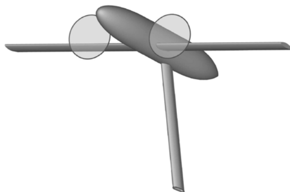
Fig. 5. A graphical representation of the aircraft configuration used to calculate engine power effects on support interference. Fuselage, wings, propeller planes and model sting are clearly discernible
