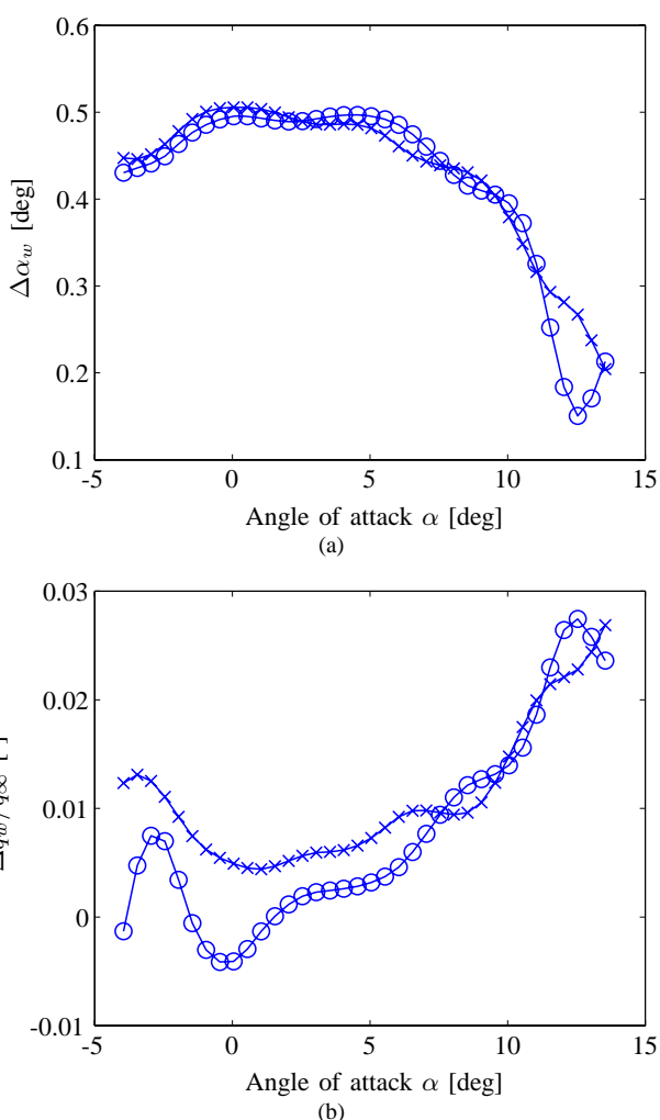
Fig. 3. Engine power effects on the values of (a) \Delta\alpha_w (b) \frac{\Delta q_w}{q_\infty} for the ventral setup of a low-speed measurement on a four-engine turboprop aircraft in the LLF of DNW. Comparison of disturbance parameters between power-off (o) and power-on (x) conditions with a moderate power setting
