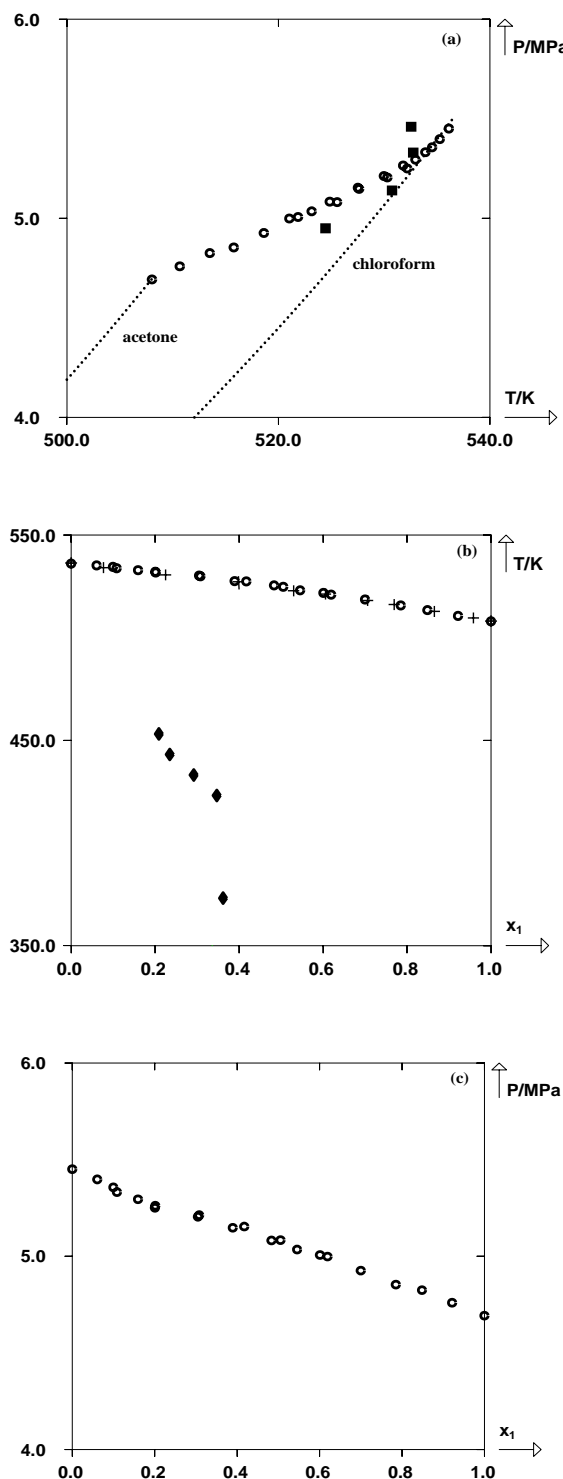
Fig. 3 Experimental critical points and critical locus in the (a): (P-T), (b): (T- x_1 ) and (c): (P- x_1 ) projections for the binary system acetone (1) + chloroform (2). Critical values (○): this work, (■): Kuenen and Robson, (+): Campbell and Musbally and azeotrope compositions (◆): Campbell and Musbally.
