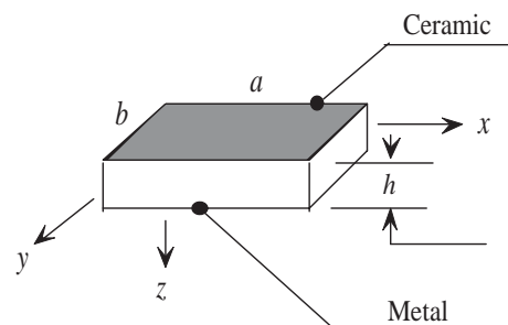
Fig. 1. Schematic diagram and dimensions of the plate.
