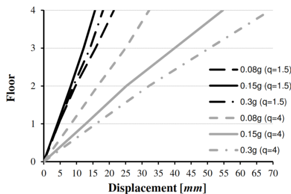
Fig. 10 Deformations of four-storey buildings in X direction (95-year return period seismic event)
