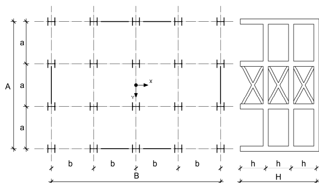
Fig. 1 Schematic plan of the studied structures
