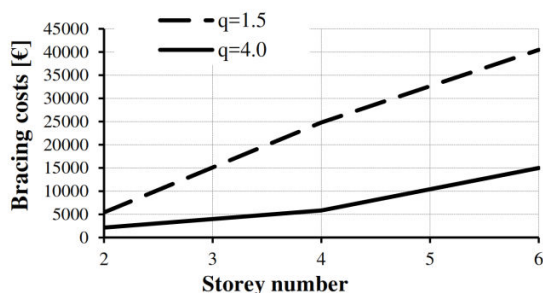
Fig. 7 Bracing costs (0.15g)
