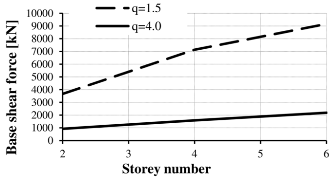
Fig. 5 Base shear forces (0.15g)
