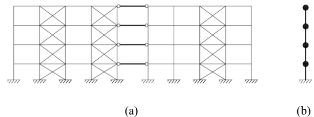
Fig. 2 Numerical model (a) approximate 2D model (b) MDOF beam model
