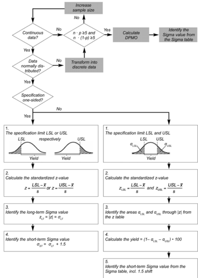
Fig. 8 Z Method for Calculating Sigma Quality Level
