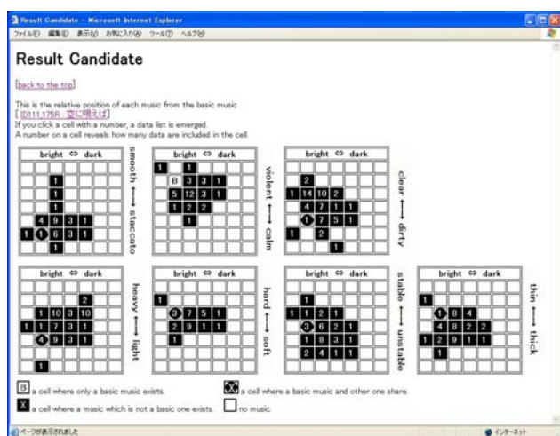
Fig. 2 Retrieval interface 2D-RIB in the paper [7]
