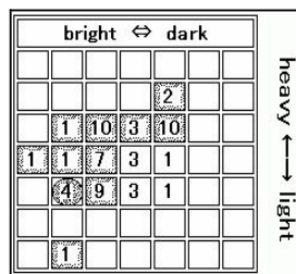
Fig. 4 One of the seven grids in Method 1
