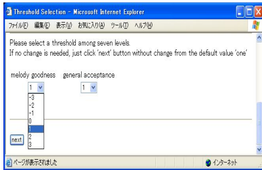
Fig. 13 Customization menu 1
