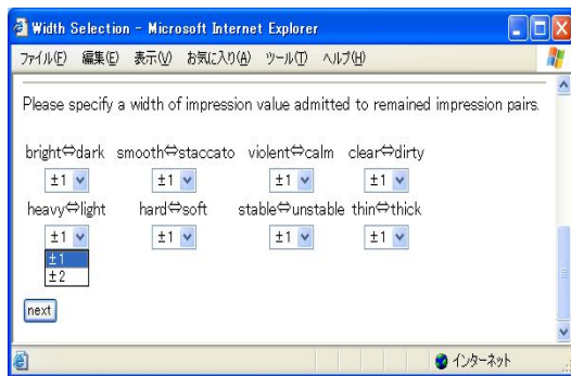
Fig. 14 Customization menu 2
