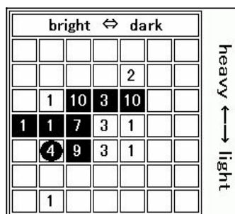
Fig. 9 One of the seven grids in Method 4
