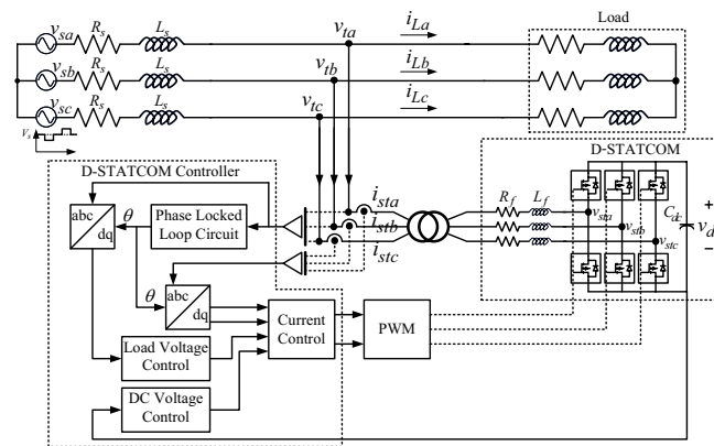
Fig. 9 Distribution system with the installed D-STATCOM
