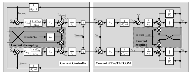
Fig. 3 Current Control structure for the D-STATCOM
