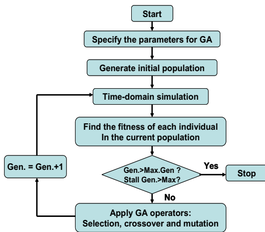
Fig. 6 Flowchart of GAs procedures
