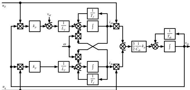
Fig. 2 Basic circuit diagram and control of the D-STATCOM system
