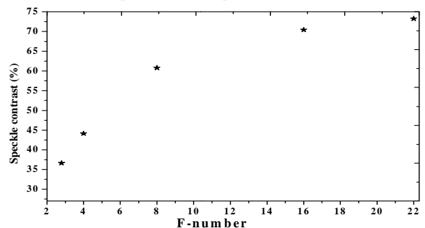
Fig. 7 Speckle contrast for different F/# of camera
